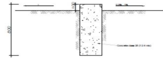
BILL CROSS SECTION B-B Scale 1:10
