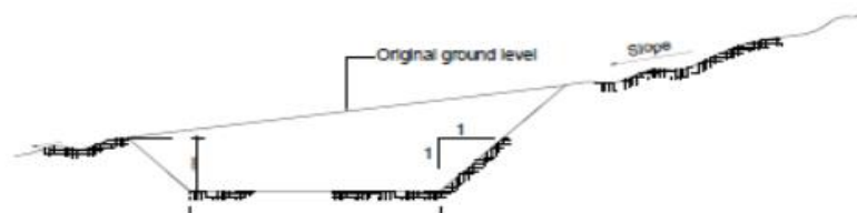
CROSS-SECTION C-C (PROTECTIVE TRENCH) Scale 1:100
