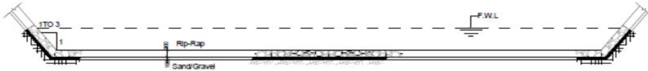
SPILLWAY PROTECTION ARRANGEMENT Scale 1:100
