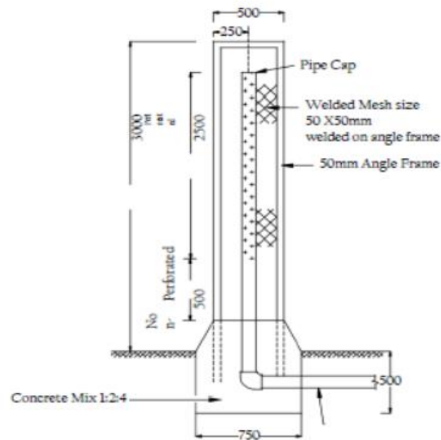
INTAKE TOWER
